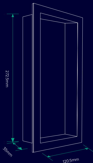
Stainless Steel Back Box
